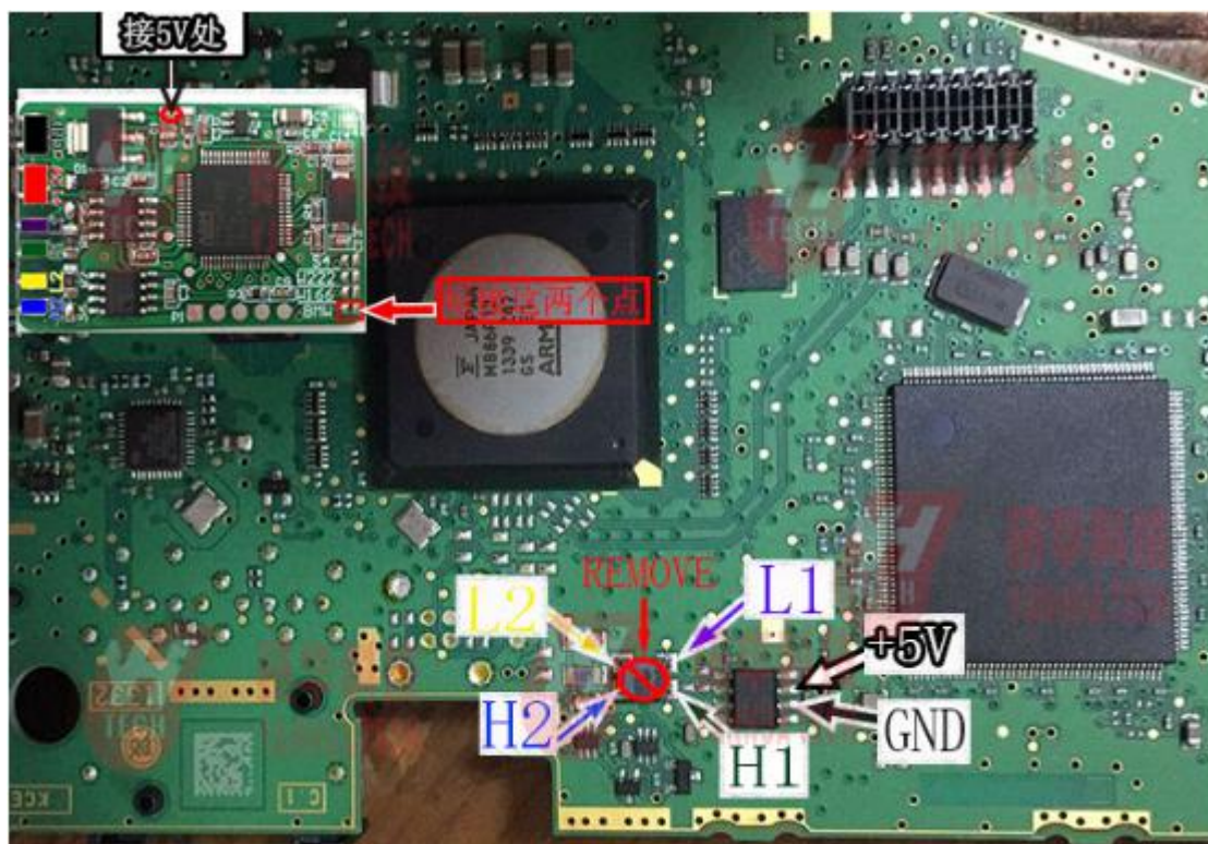
6. Below is the diagram for BMW FEM:
