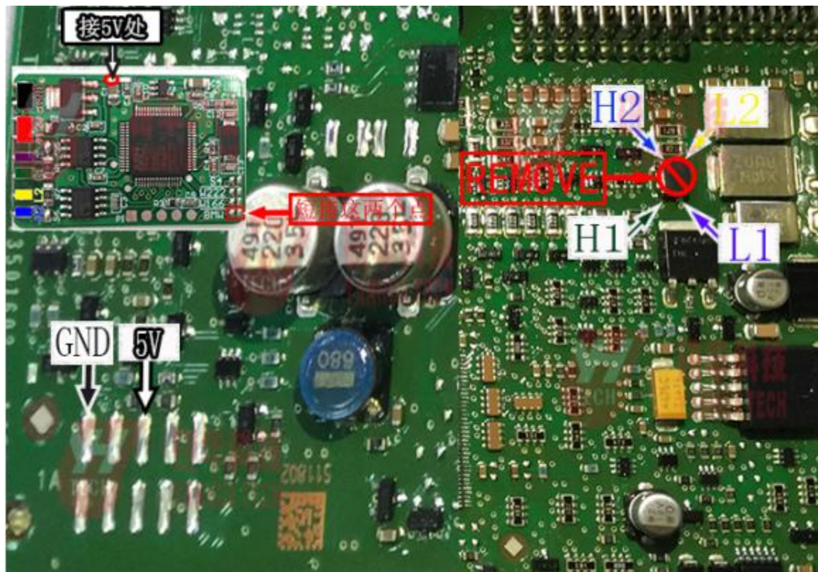
8. Below is the diagram for BMW X3 F25 instrument:
