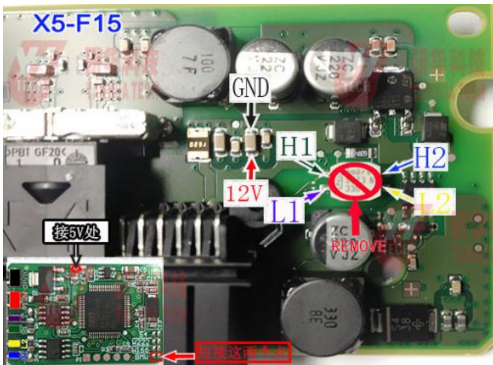
5. Below is the diagram for USA Standard BMW X5 F15 instrument:
