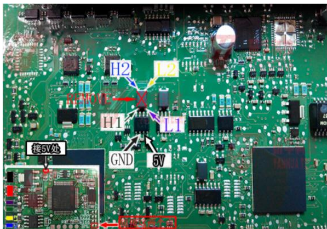
7. Below is the diagram for BMW CAS4(1L15Y/5M48H/1N35H)
